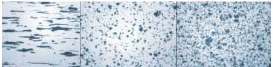
AgNi10 longitudinal section (parallel to the direction of extrusion)
